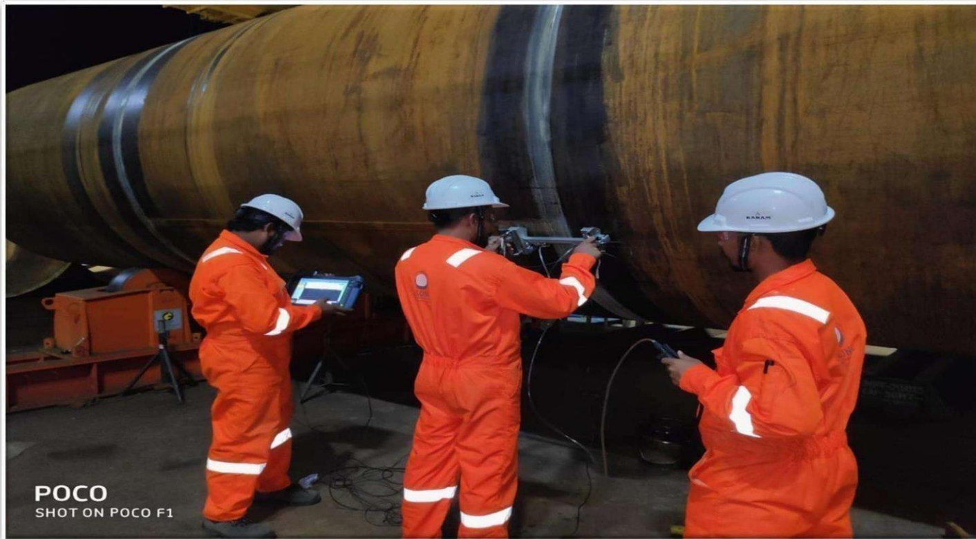
PAUT & TOFD Inspection of Structure joints at L&T MFF, Hazira
