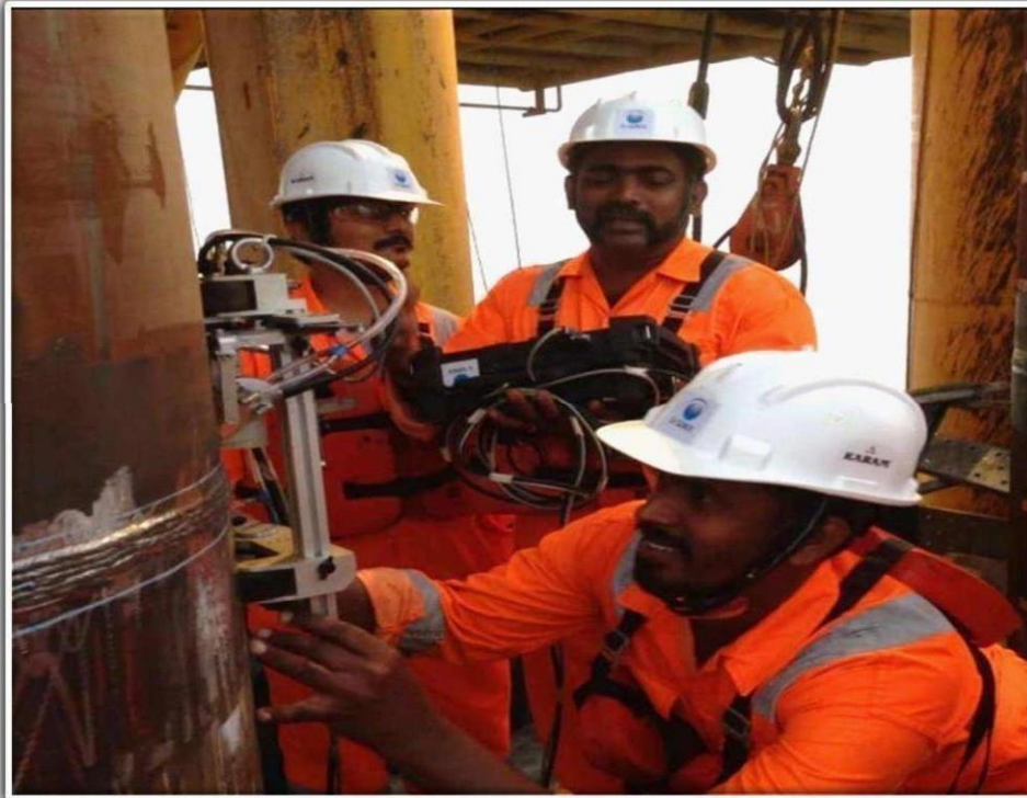
PAUT Inspection of Structure & Piping joints for L&T Offshore, ONGC Mumbai
